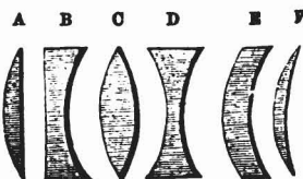
LENSES OF DIFFERENT FORMS.
