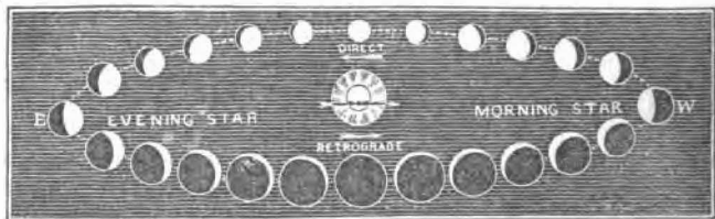
PHASES OF VENUS AS SHE REVOLVES AROUND THE SUN.
