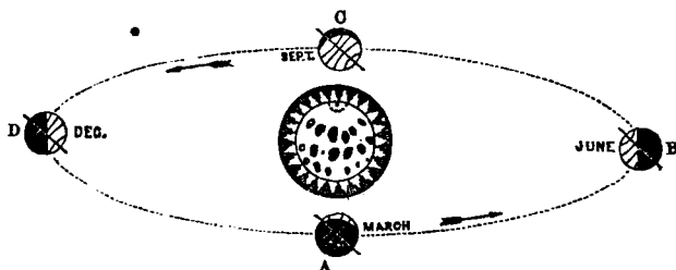
SOLAR SPOTS OBSERVED FROM DIFFERENT POSITIONS.
