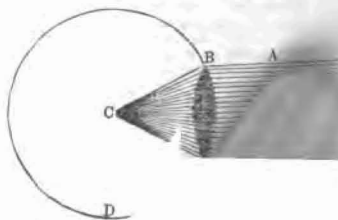
DOUBLE CONVEX—FOCAL DISTANCE.
