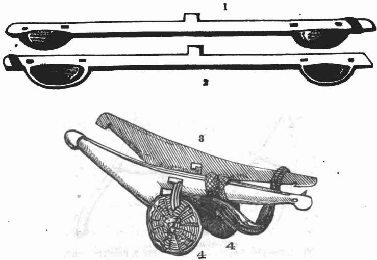
360. Yoke of an ancient plough found in a tomb. Collection of S. d'Athanas. Figs. 1, 2. The back and front of the yoke. 3. Collar or shoulder pieces attached to the yoke. 4, 4. The pieces of matting for protecting the two shoulders from friction.
