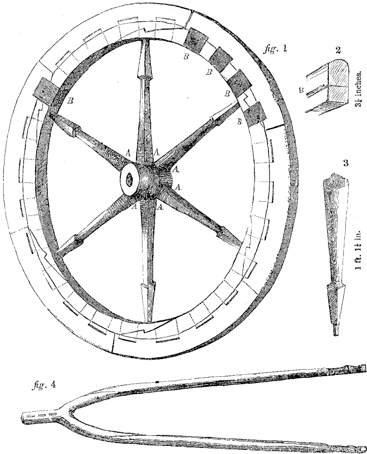
336. Fig. 1. Wheel; 3 ft. 1 in. diameter. In the Collection of Dr. Abbott. Fig. 4. Shafts; 11 feet in total length.
